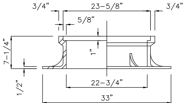
SECTION OF COVER
