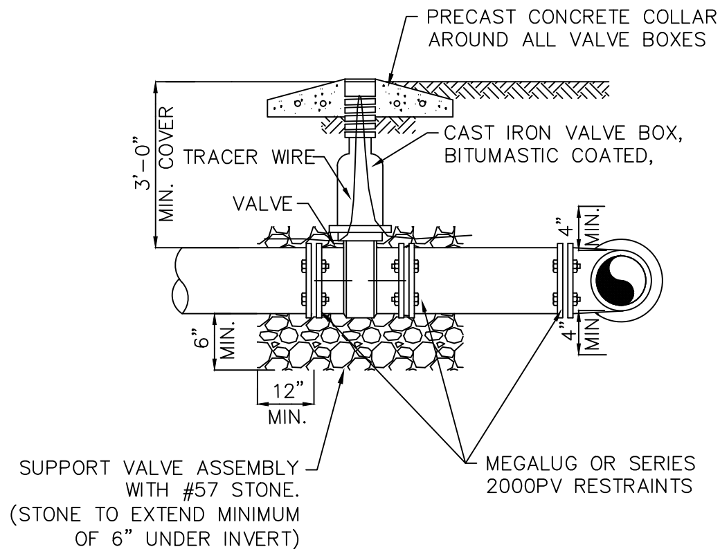
VALVE & TEE SETTING DETAIL NOT TO SCALE
